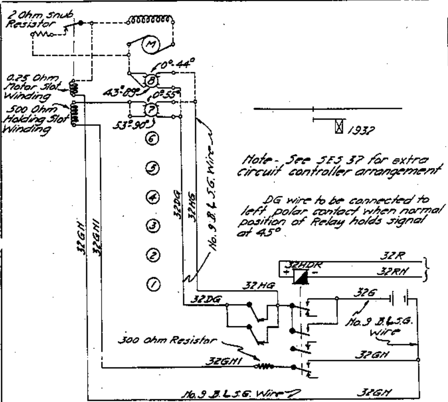
LOCAL WIRING FOR 3 POSITION STYLE T2 SIGNAL WITH POLARIZED CONTROL When it is not desired to hold signal cleared from line circuit:
